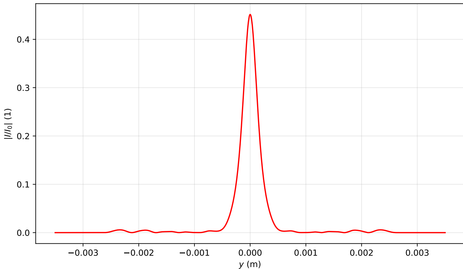
Intensity profile I(x=0, y, z=2.866)/I_0 , \text{Pin}=7.0\text{Pcr} , artificial time
